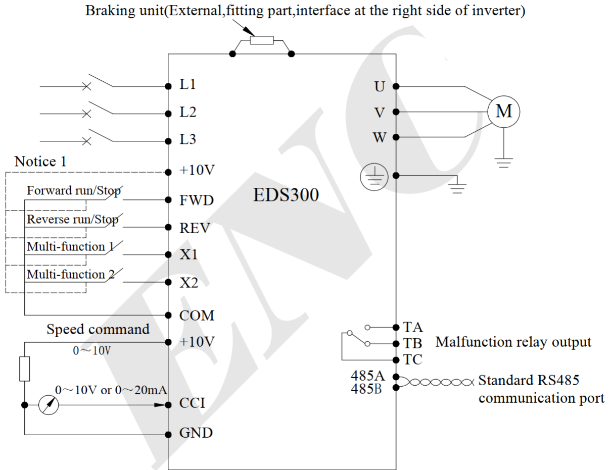
Fig. 3-6 Basic wiring diagram
